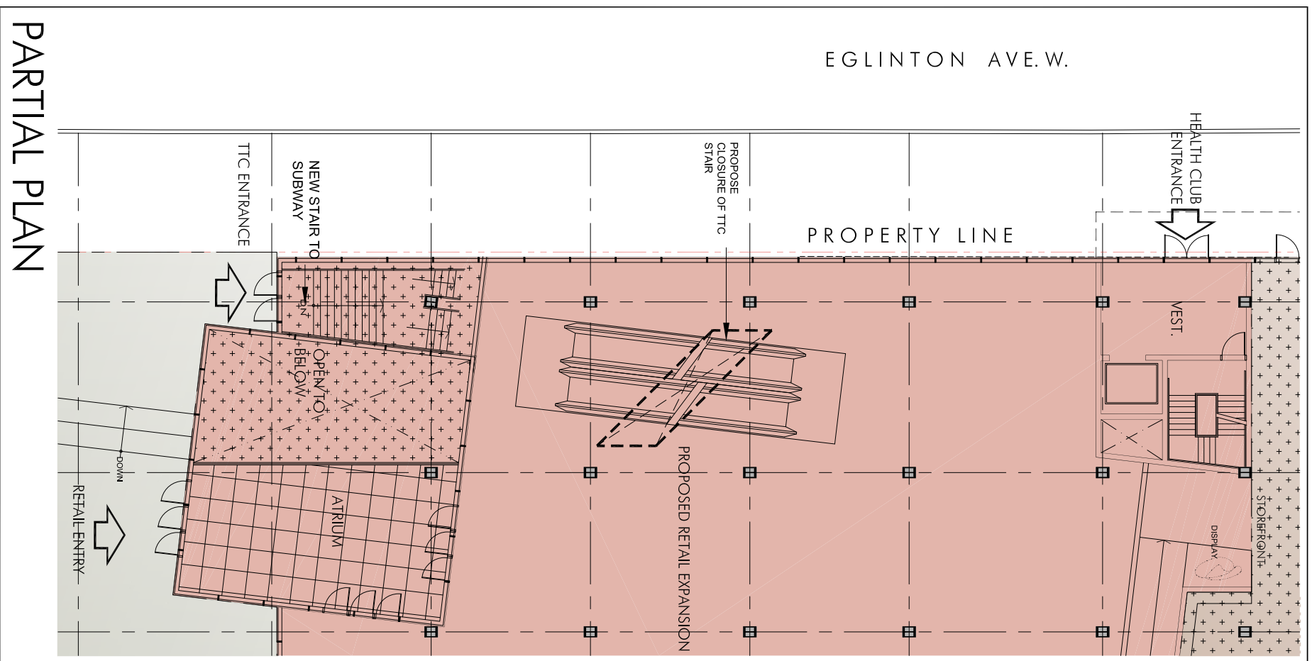
PARTIAL PLAN
